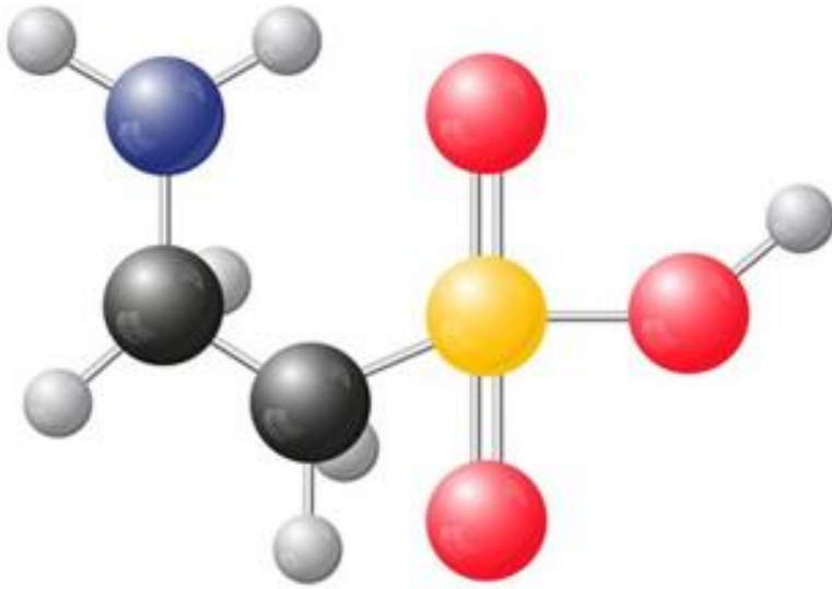
Taurine
